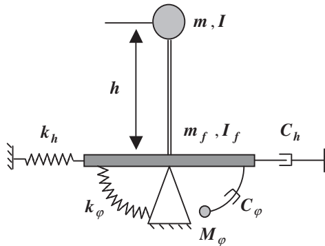
Figure 2: Soil-structure model
